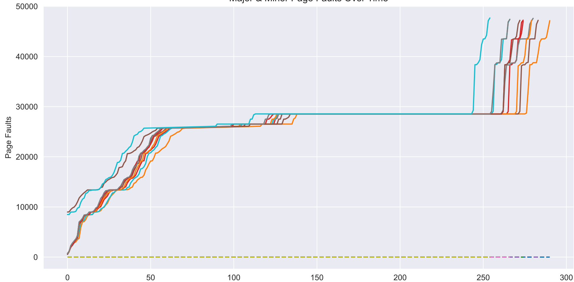
Major & Minor Page Faults Over Time
