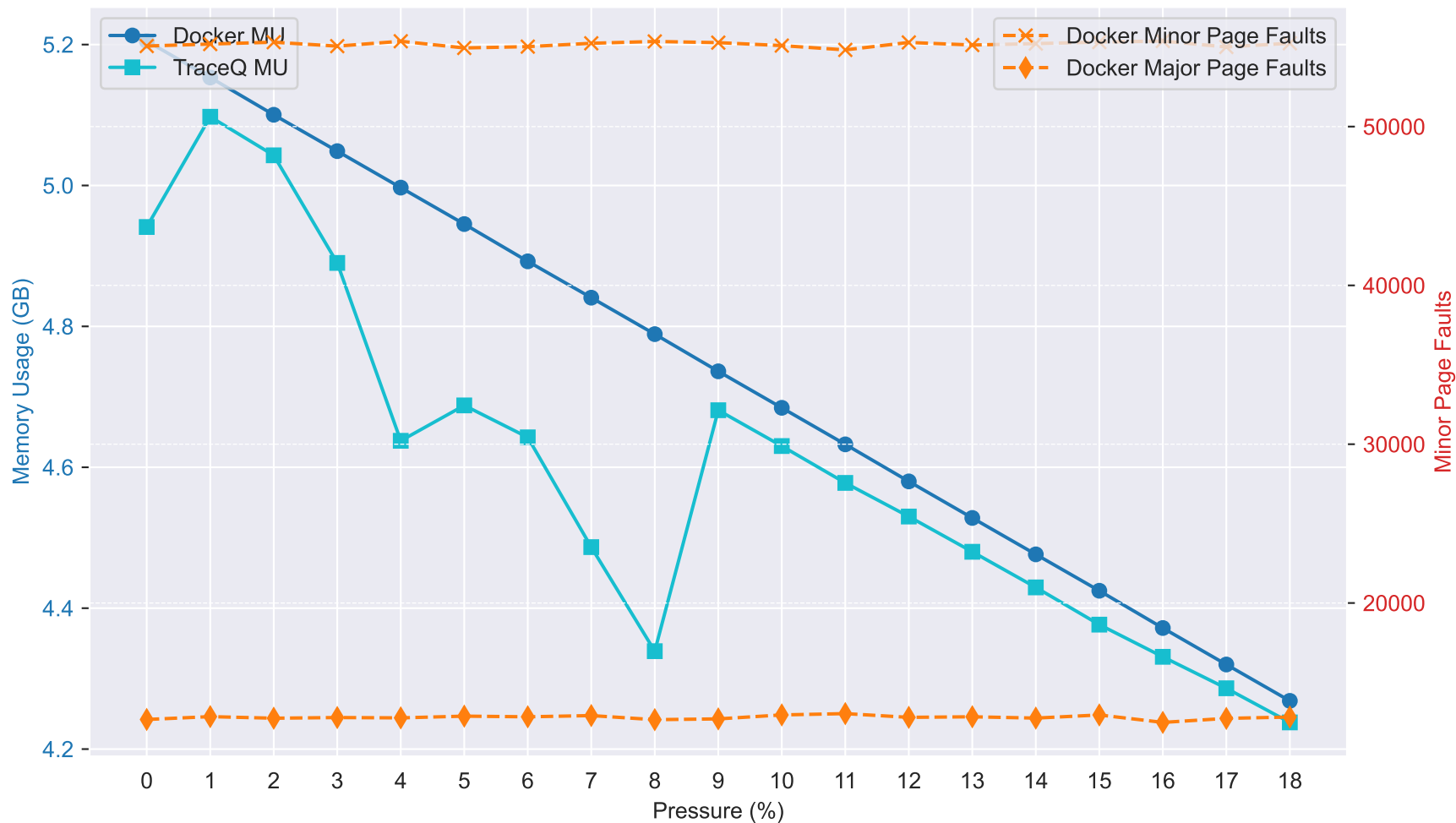
Memory Usage and Page Faults per Profile
