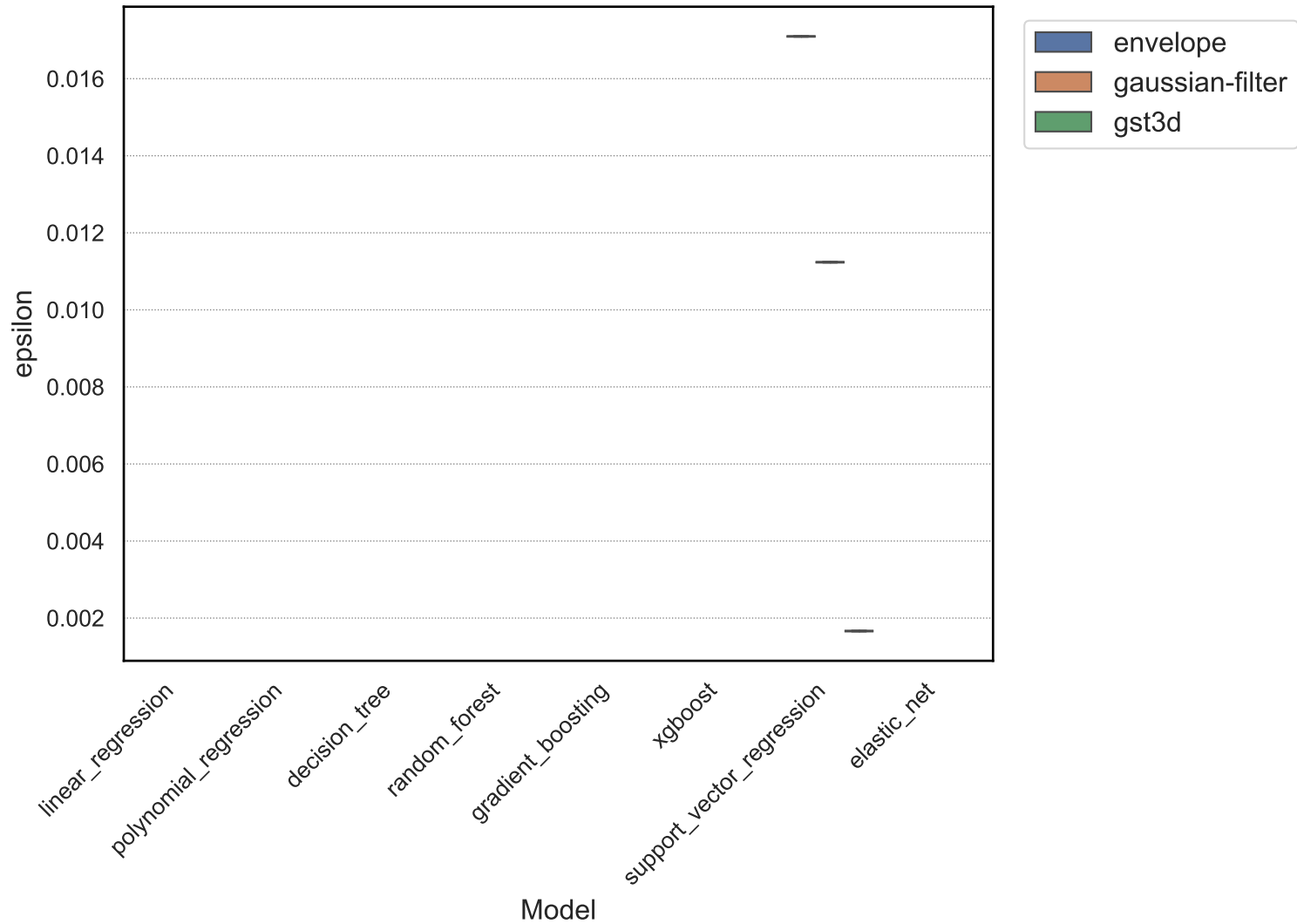
Hyperparam Distribution - epsilon
