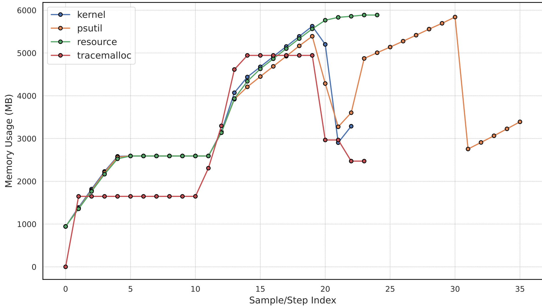
Memory Usage History by Tool (No TraceQ)
