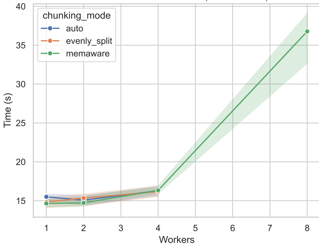
Execution Time vs Workers (200x200x200)
