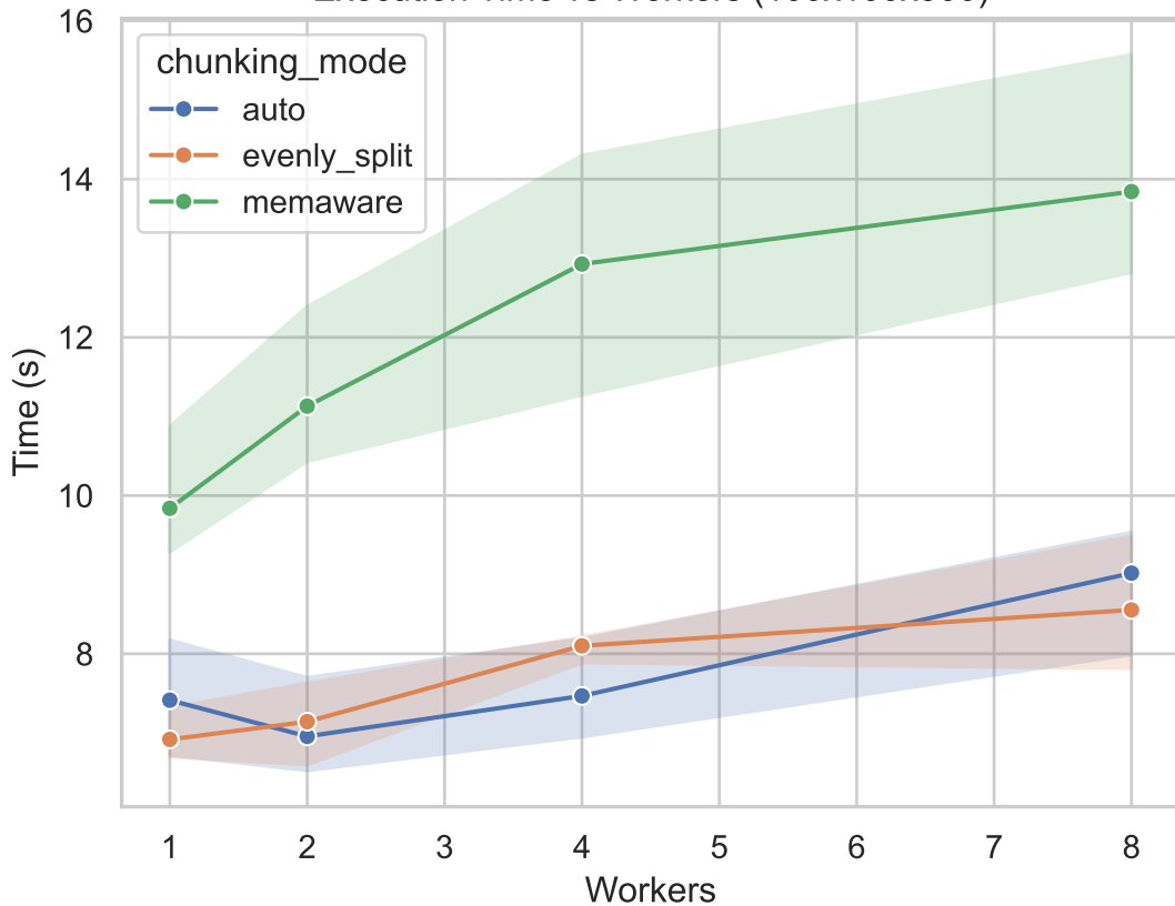
Execution Time vs Workers (100x100x300)
