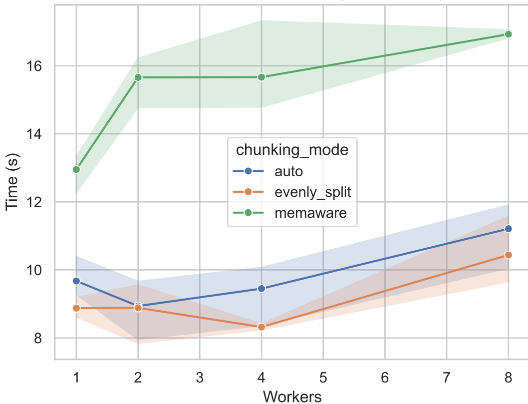
Execution Time vs Workers (100x100x400)
