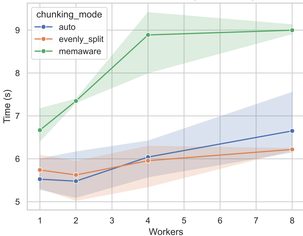
Execution Time vs Workers (100x200x100)
