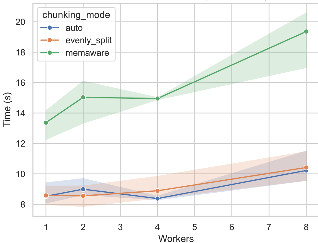
Execution Time vs Workers (100x200x200)
