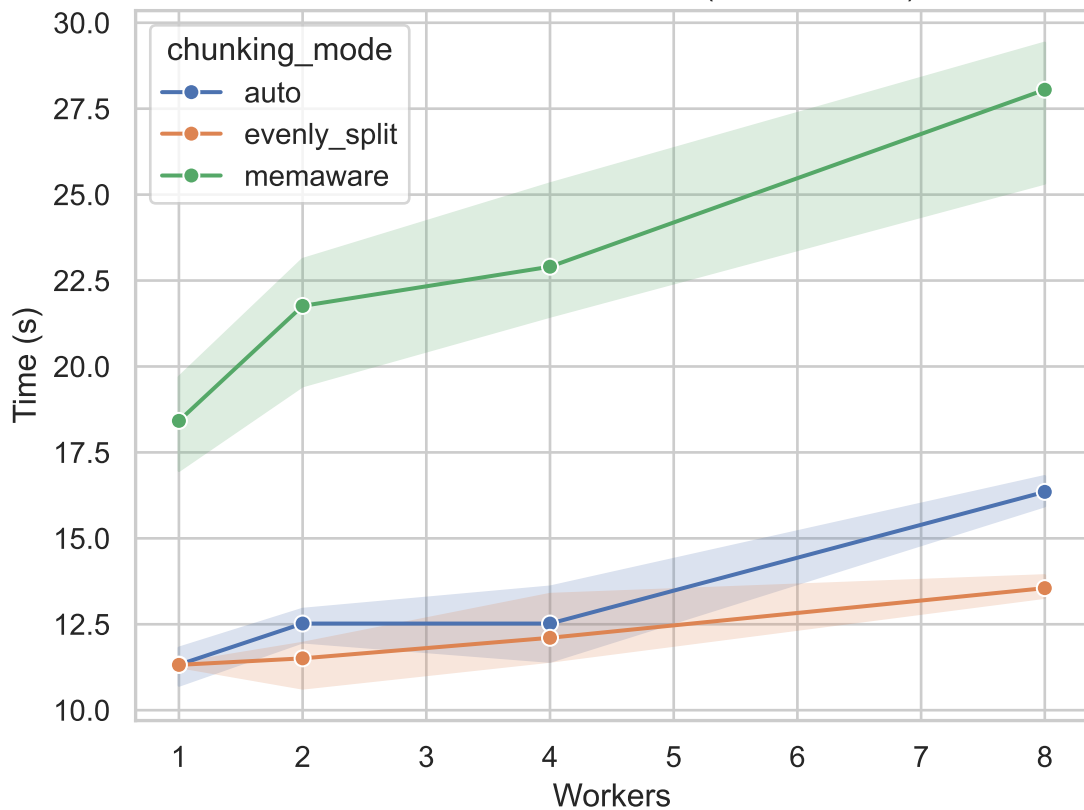
Execution Time vs Workers (100x200x300)
