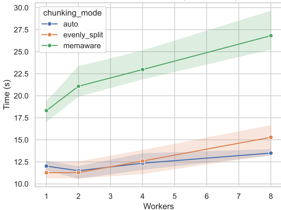
Execution Time vs Workers (100x300x200)
