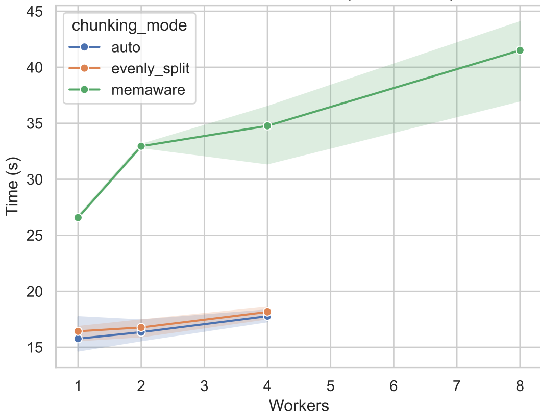
Execution Time vs Workers (100x300x300)
