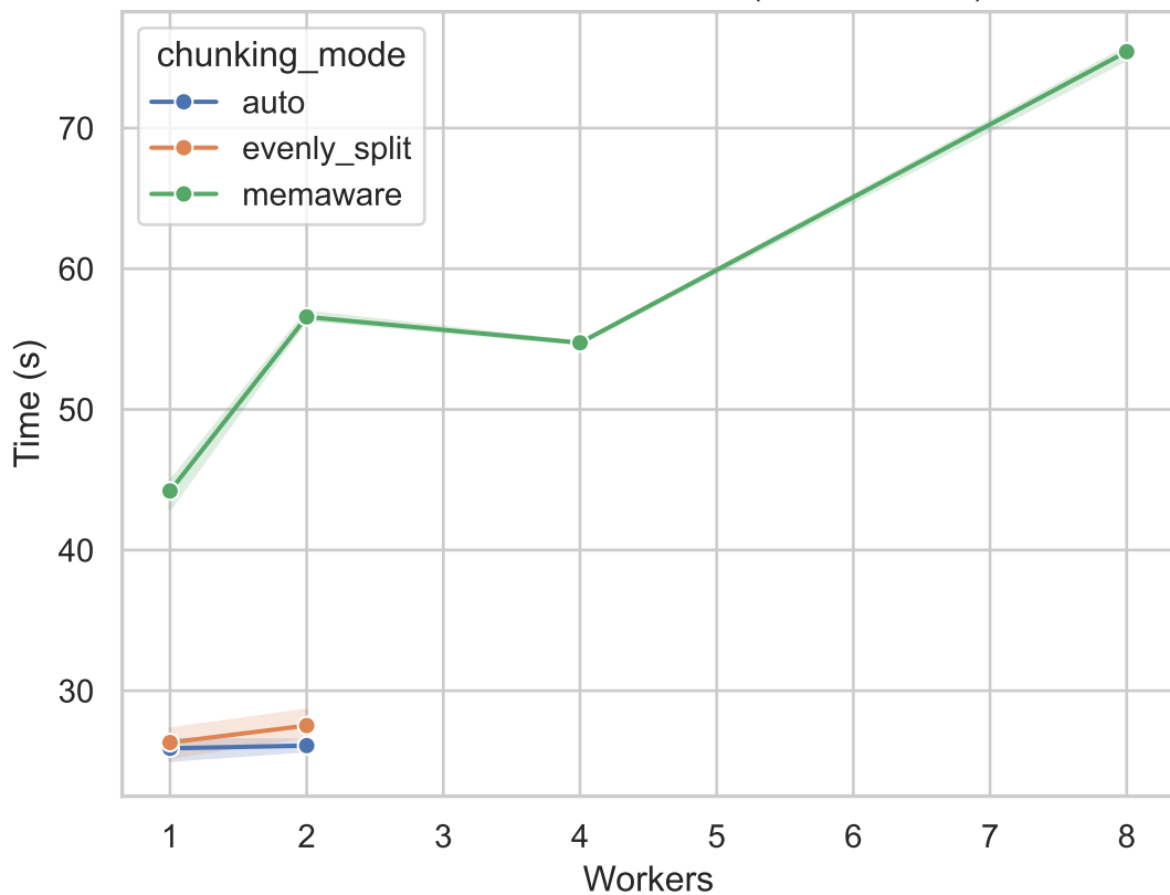
Execution Time vs Workers (100x400x400)
