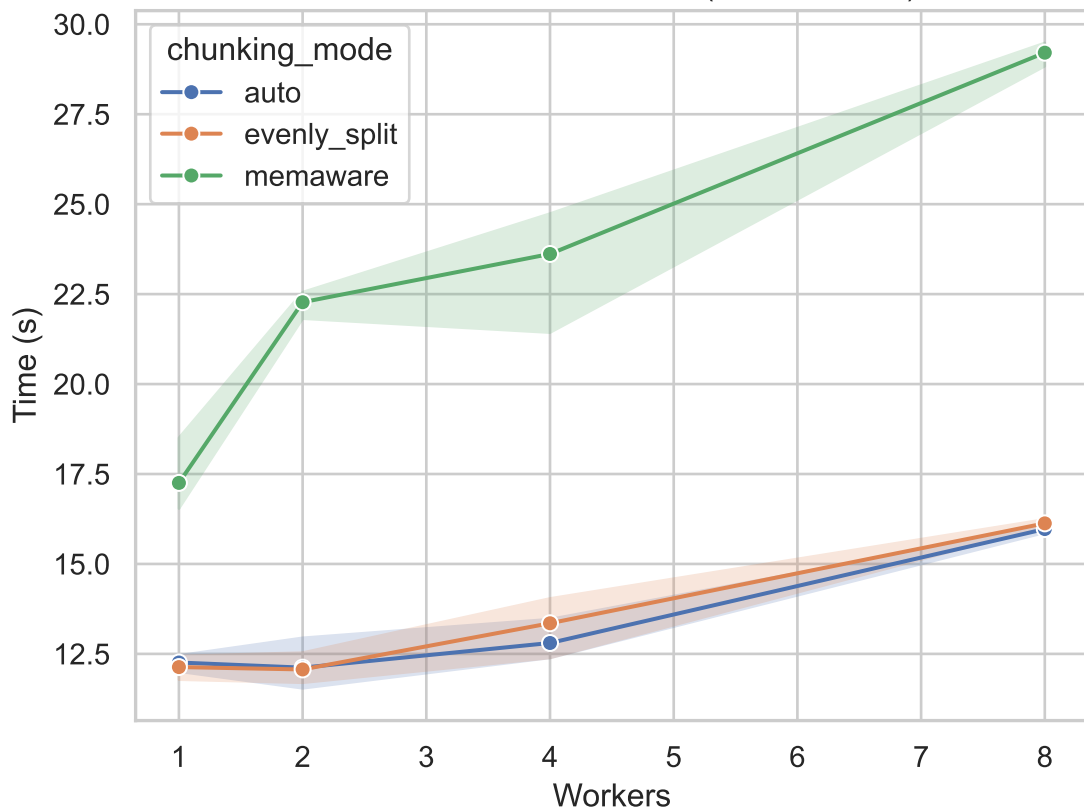
Execution Time vs Workers (200x100x300)
