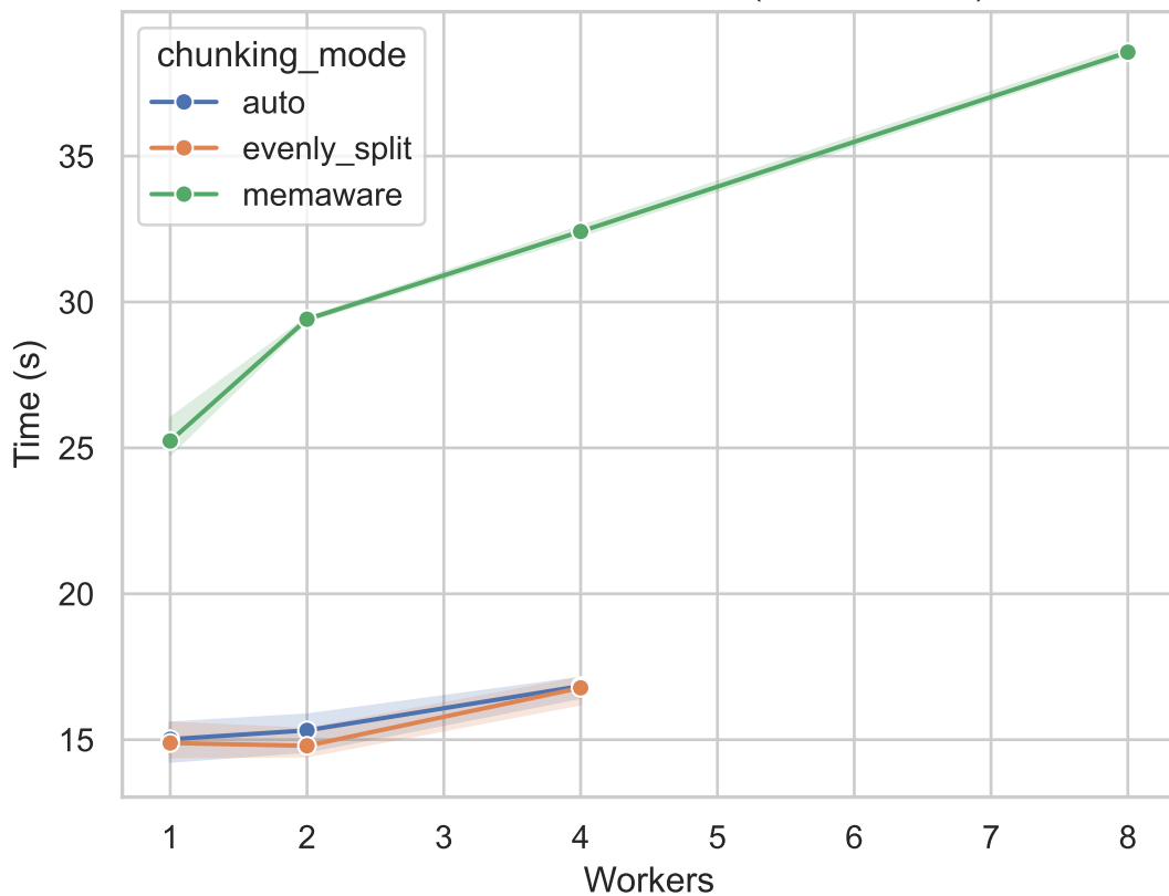
Execution Time vs Workers (200x100x400)
