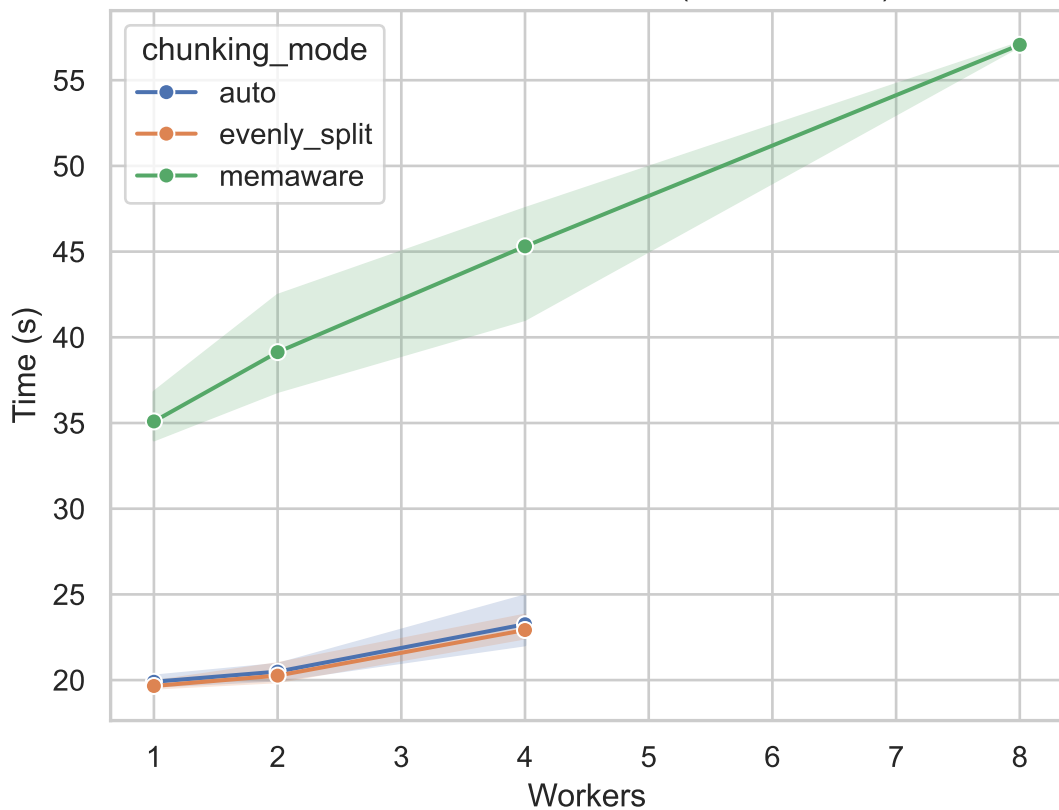
Execution Time vs Workers (200x300x200)
