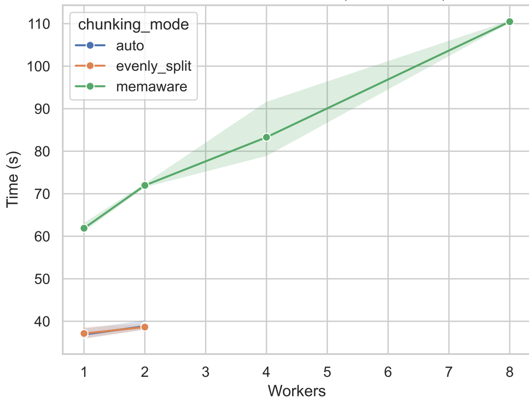
Execution Time vs Workers (200x300x400)
