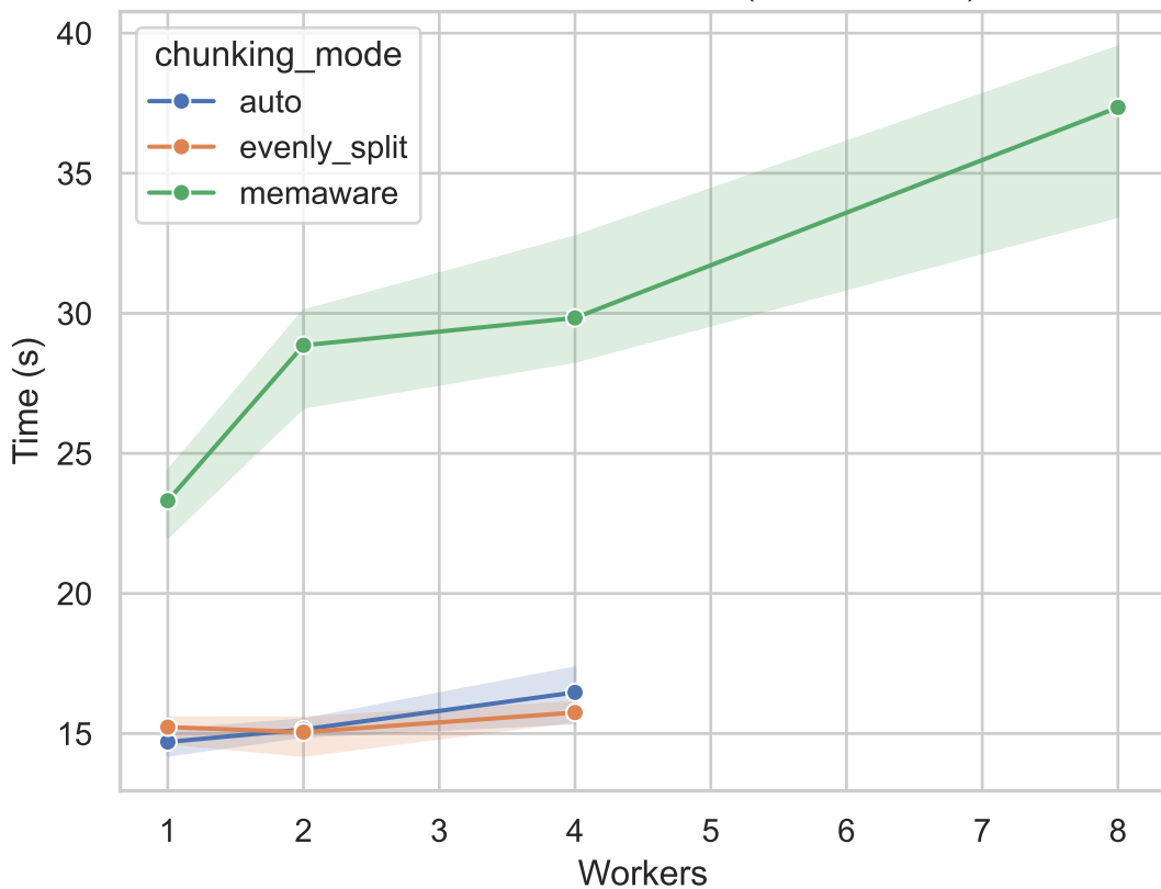
Execution Time vs Workers (200x400x100)
