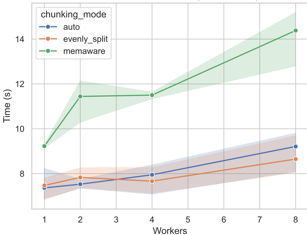
Execution Time vs Workers (300x100x100)
