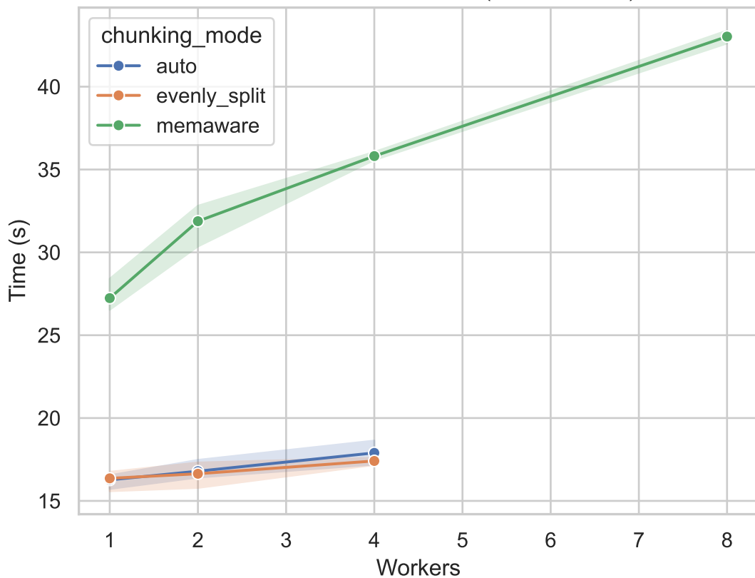
Execution Time vs Workers (300x100x300)
