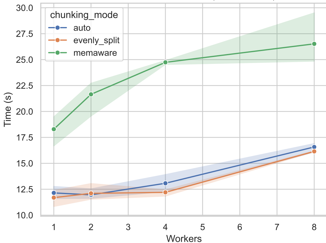
Execution Time vs Workers (300x200x100)
