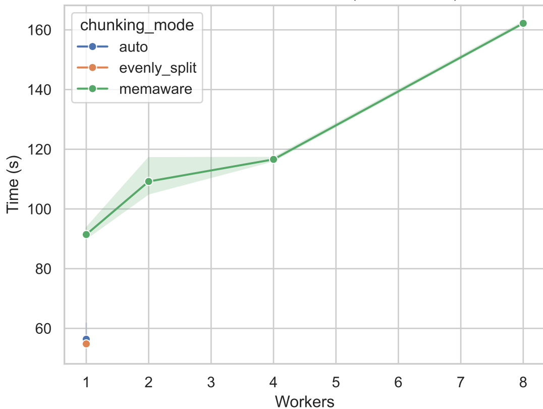
Execution Time vs Workers (300x300x400)
