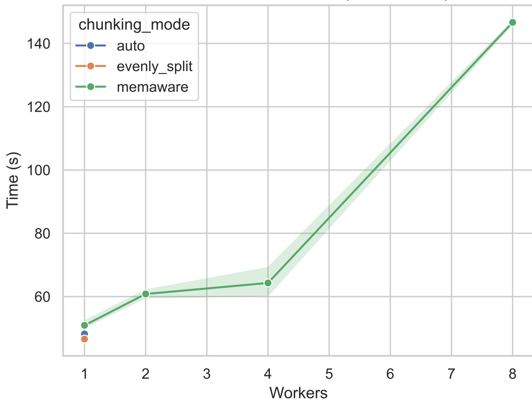
Execution Time vs Workers (400x400x200)
