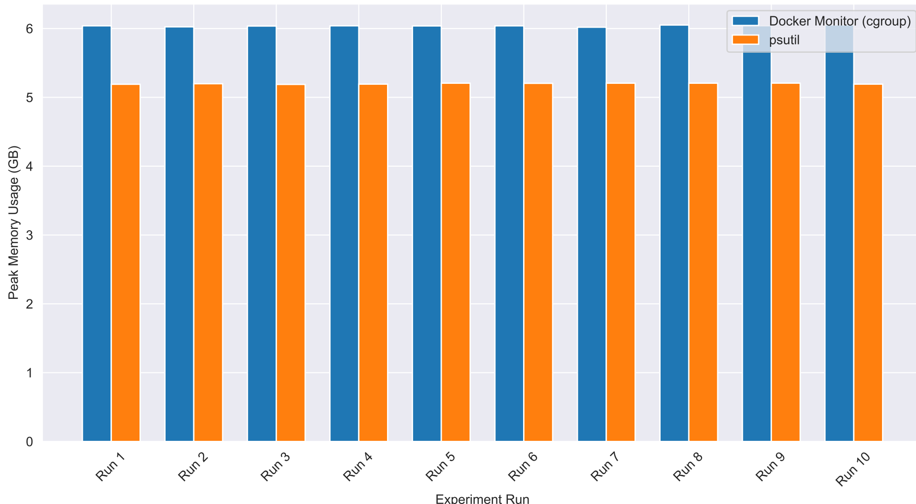
Peak Memory Usage Comparison
