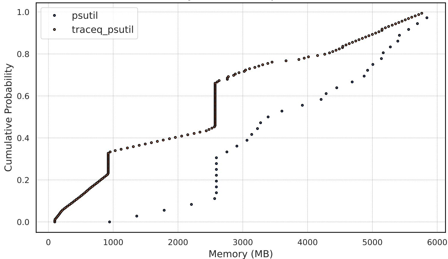
CDF Memory Distribution: psutil vs TraceQ
