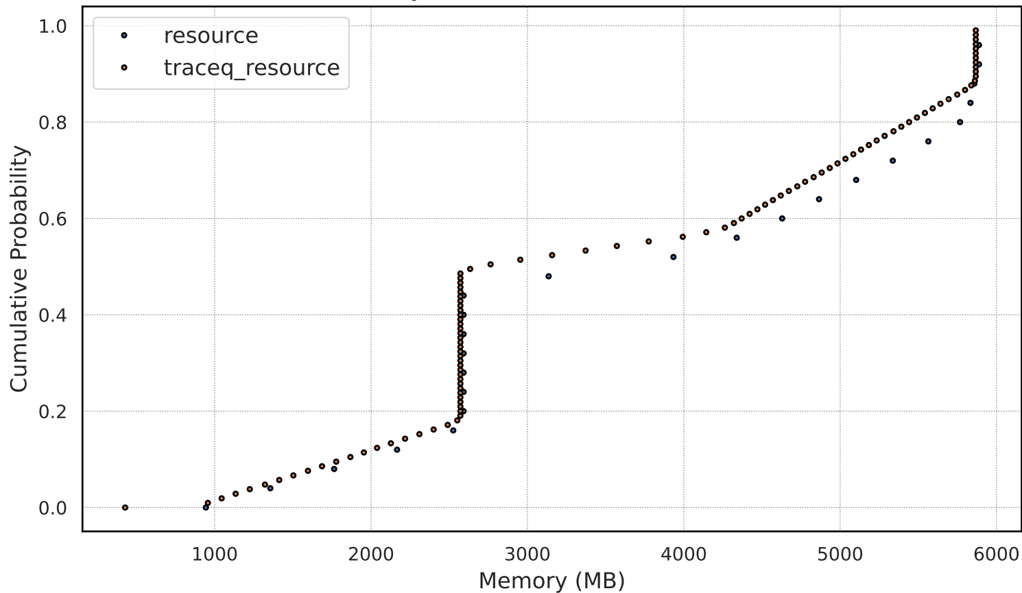
CDF Memory Distribution: resource vs TraceQ
