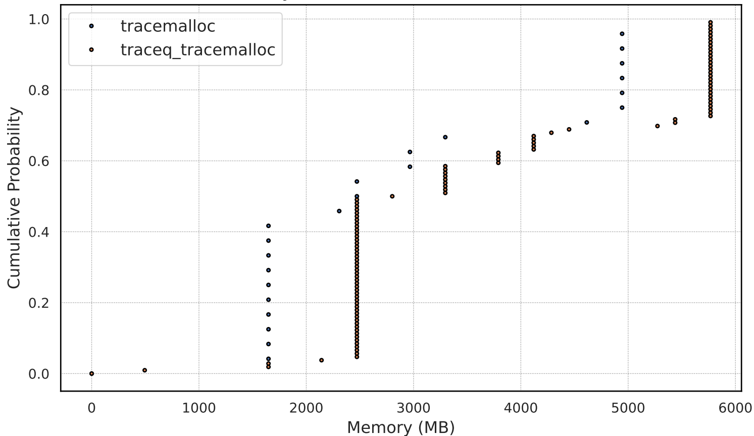
CDF Memory Distribution: tracemalloc vs TraceQ
