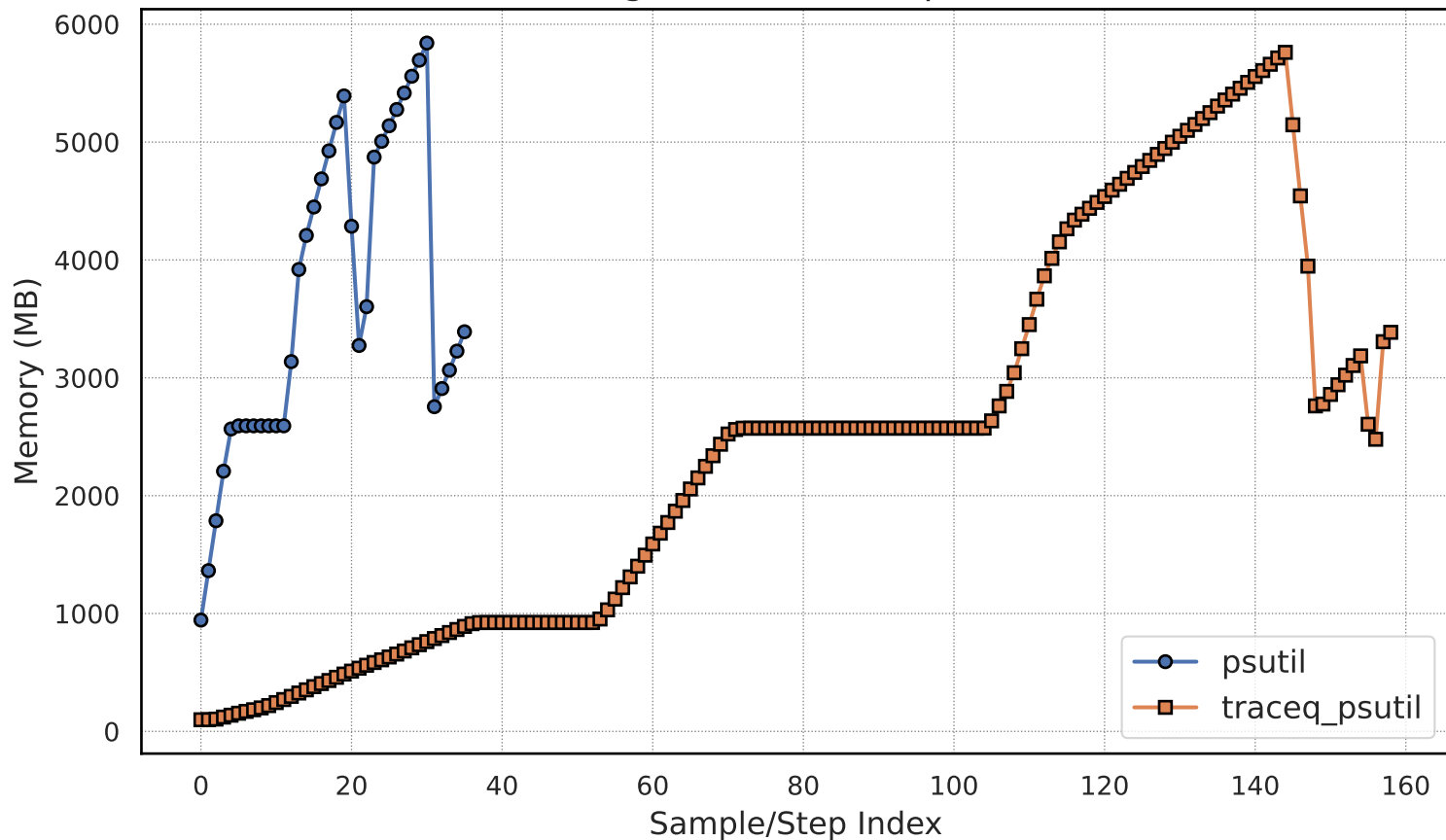
Original vs TraceQ: psutil
