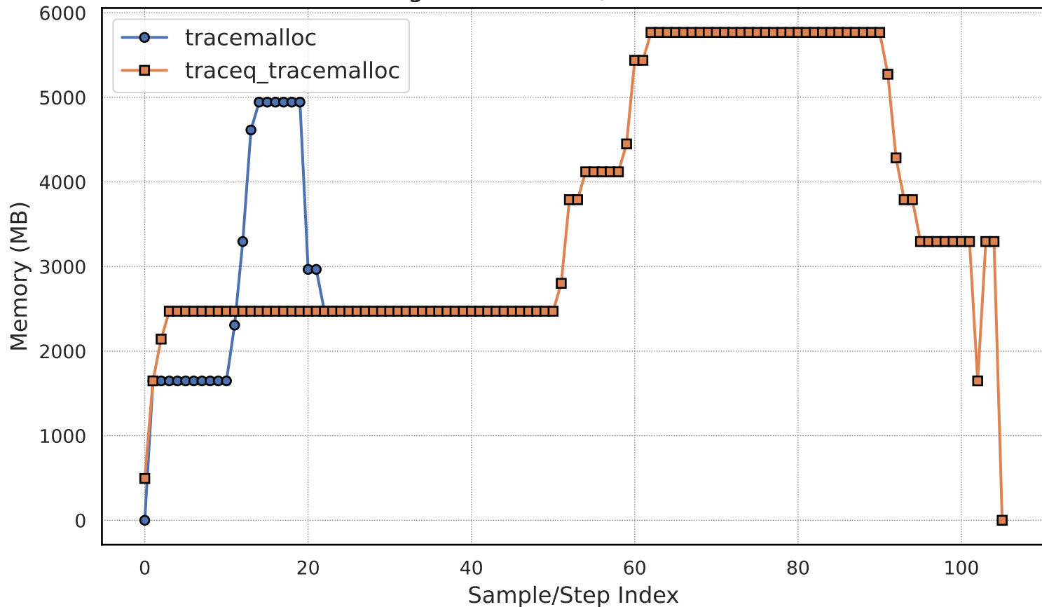
Original vs TraceQ: tracemalloc
