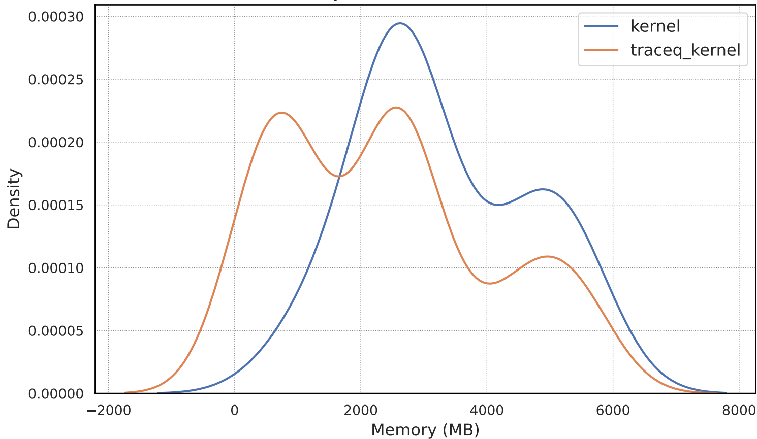
KDE Memory Distribution: kernel vs TraceQ
