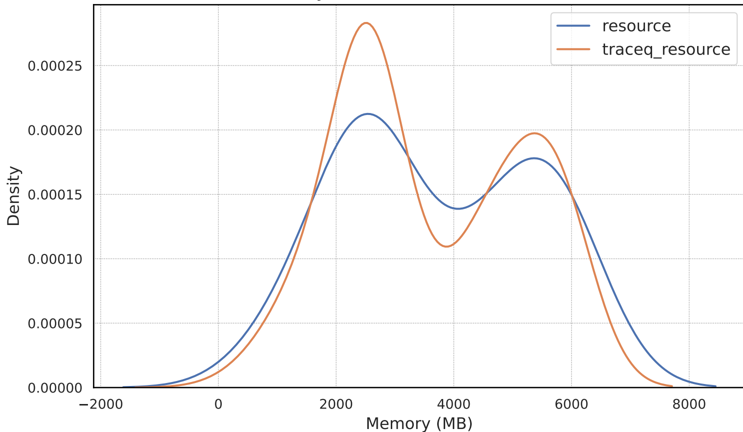
KDE Memory Distribution: resource vs TraceQ
