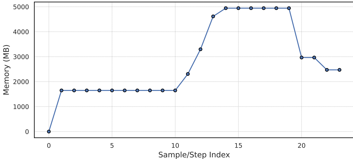
tracemalloc Memory Usage History
