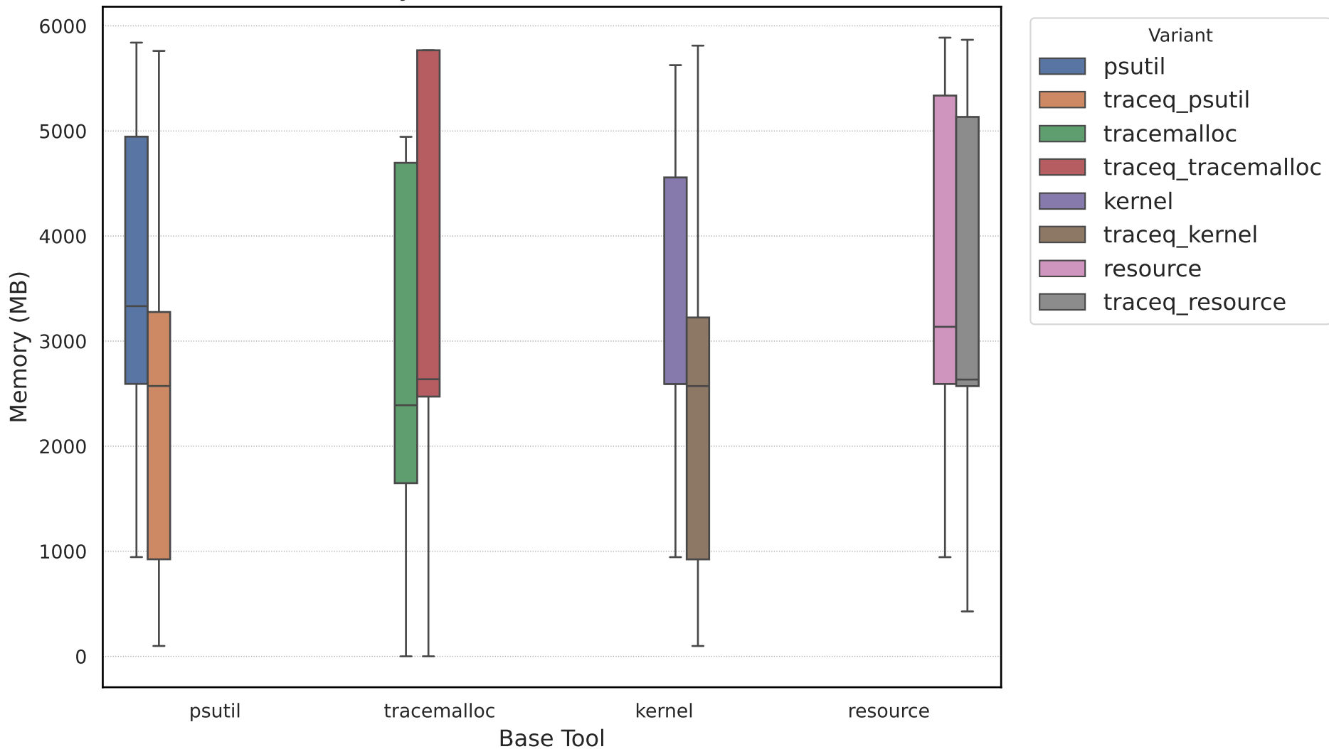
Memory Distribution: Base vs TraceQ
