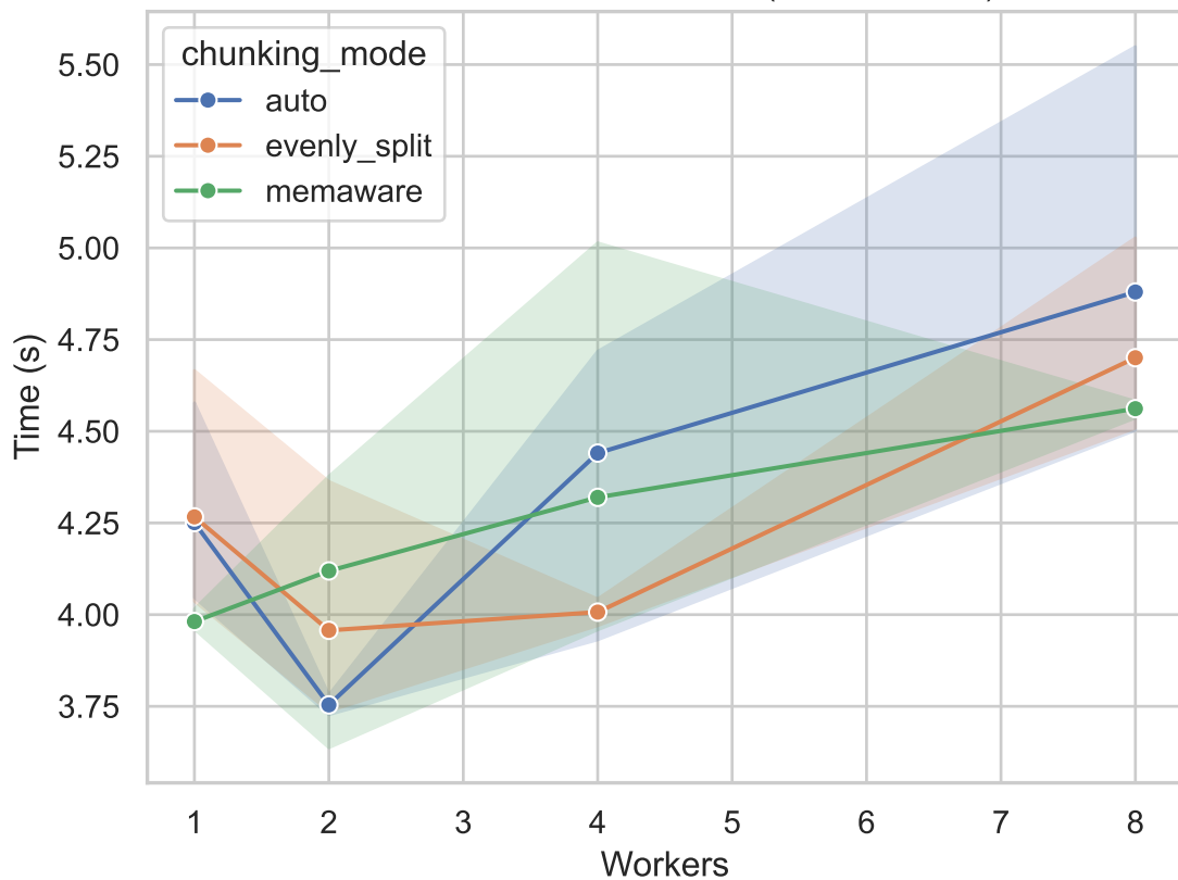
Execution Time vs Workers (100x100x100)
