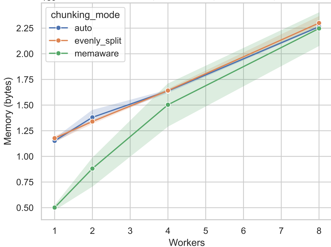
1e9 Peak Memory vs Workers (100x200x200)
