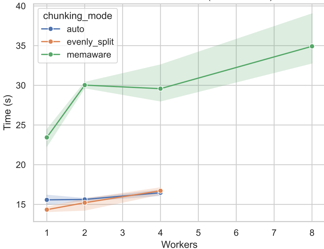
Execution Time vs Workers (100x200x400)
