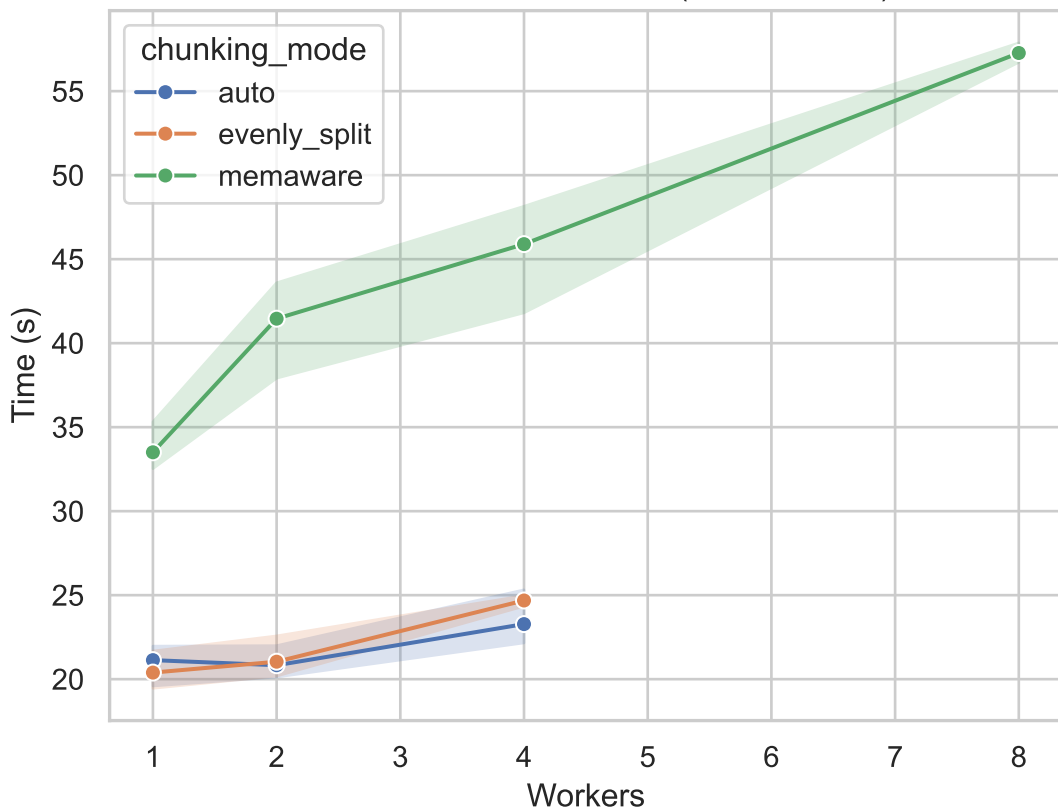
Execution Time vs Workers (100x300x400)
