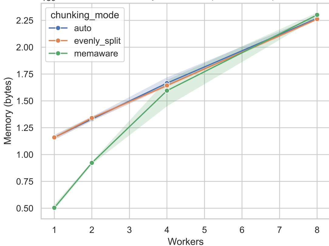
1e9 Peak Memory vs Workers (100x400x100)
