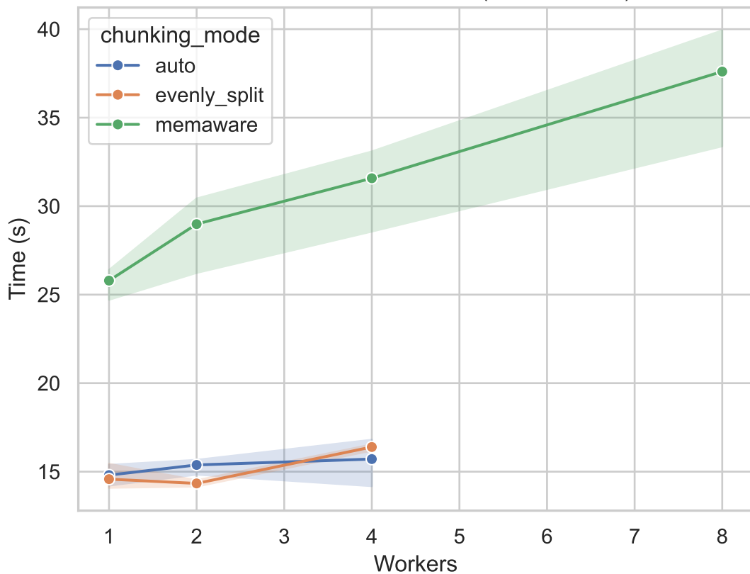
Execution Time vs Workers (100x400x200)
