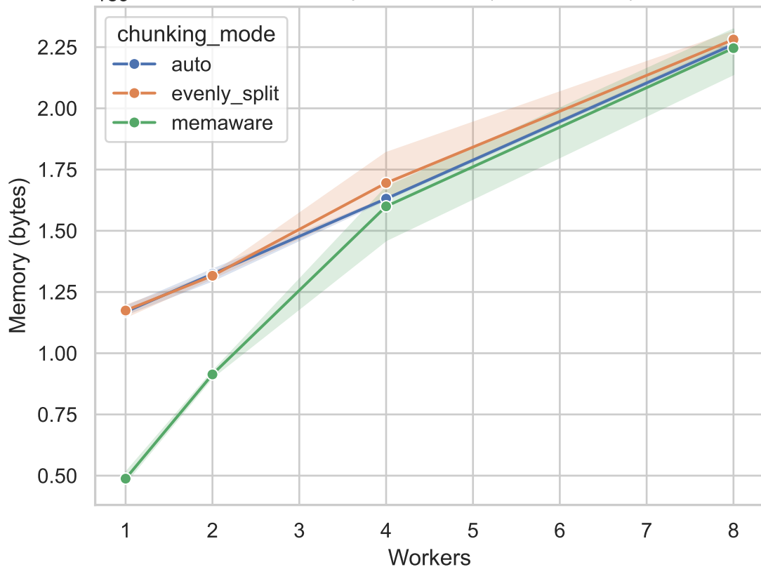
1e9 Peak Memory vs Workers (200x100x200)
