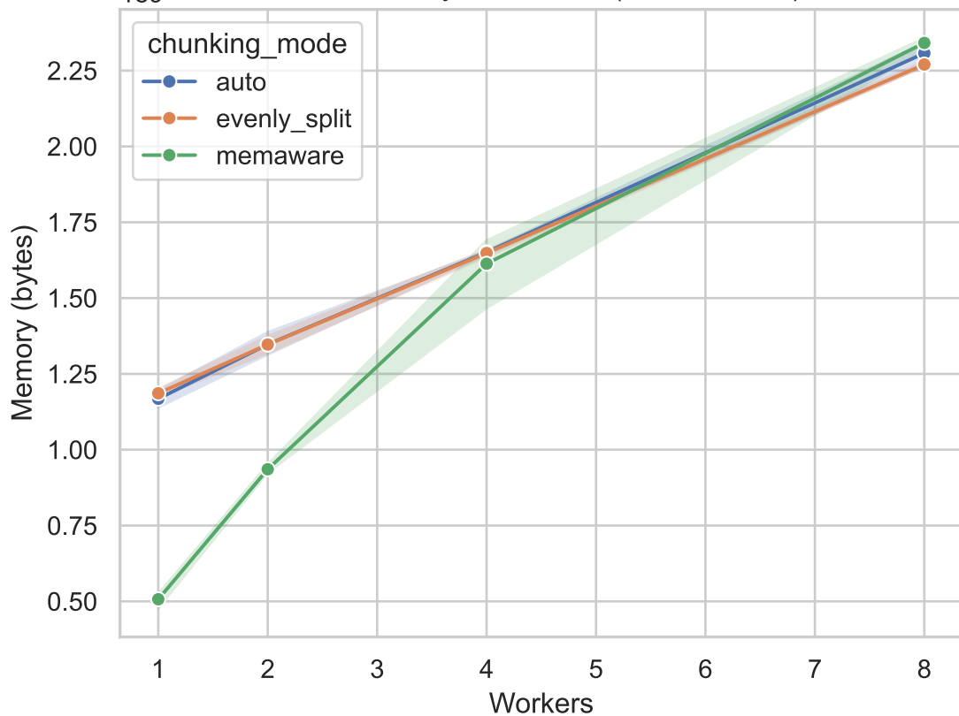
1e9 Peak Memory vs Workers (200x200x100)
