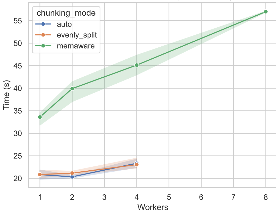
Execution Time vs Workers (200x200x300)
