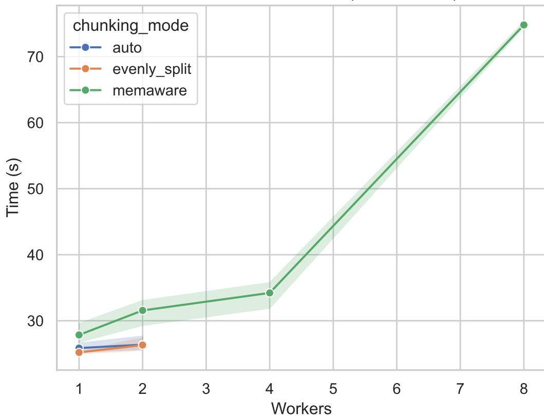
Execution Time vs Workers (200x400x200)
