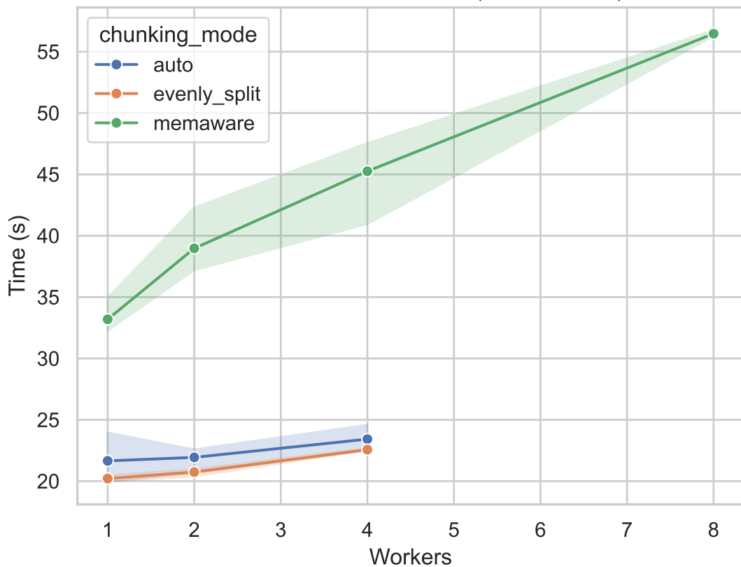
Execution Time vs Workers (300x100x400)
