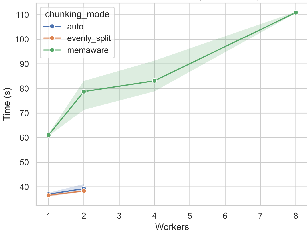
Execution Time vs Workers (300x200x400)
