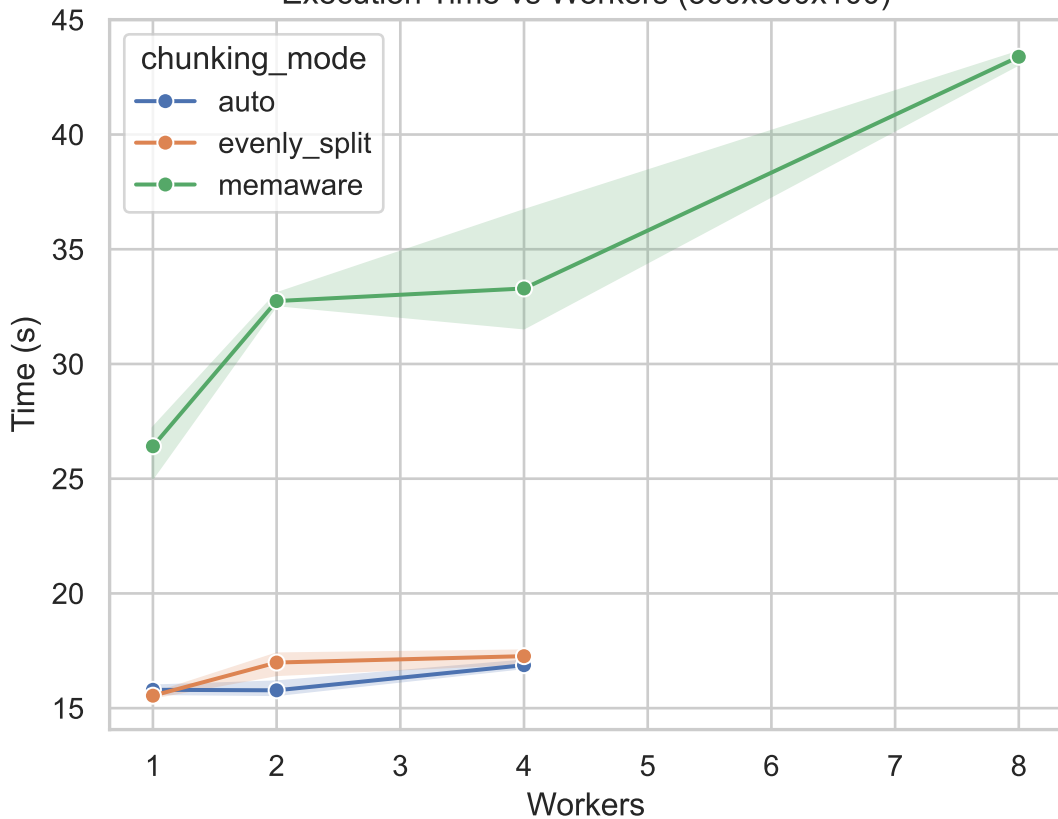
Execution Time vs Workers (300x300x100)
