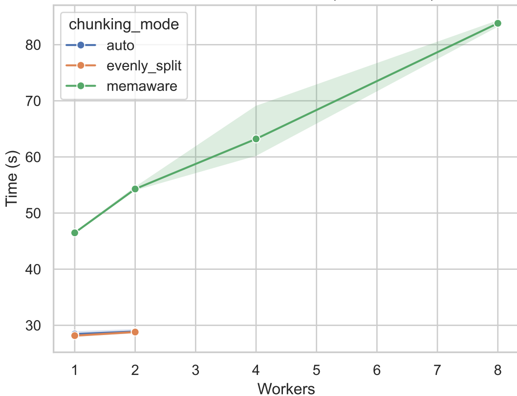
Execution Time vs Workers (300x300x200)
