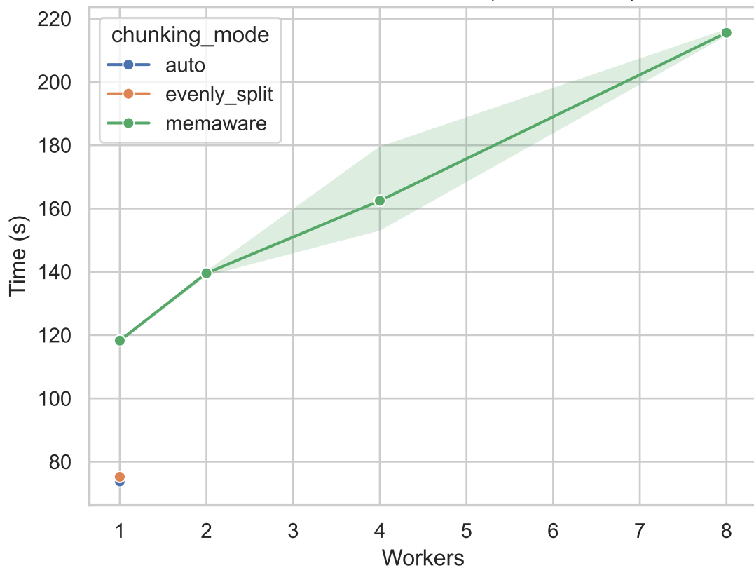
Execution Time vs Workers (300x400x400)
