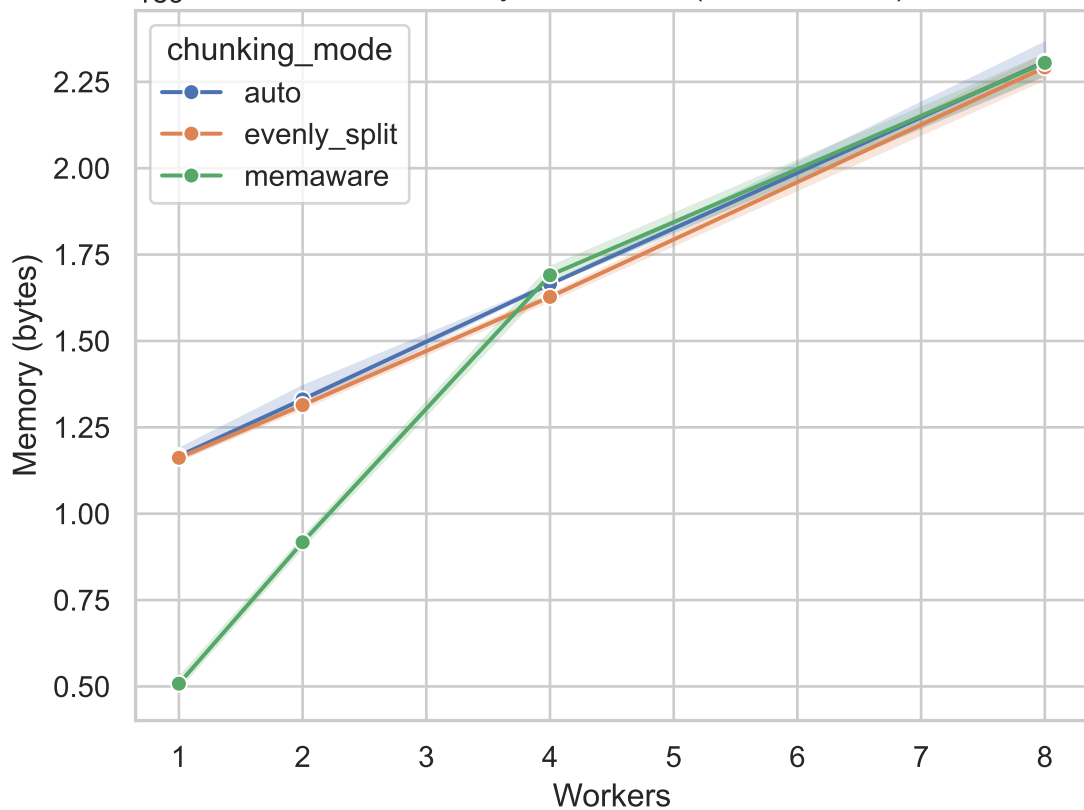
1e9 Peak Memory vs Workers (400x100x100)
