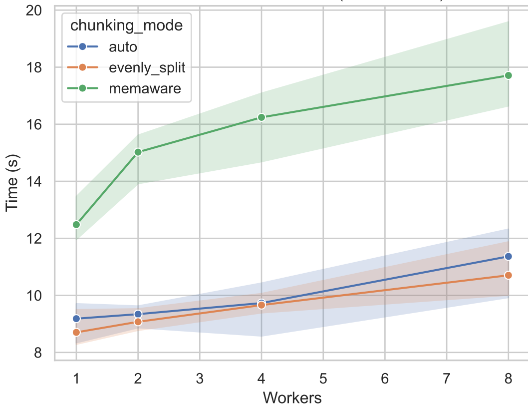
Execution Time vs Workers (400x100x100)
